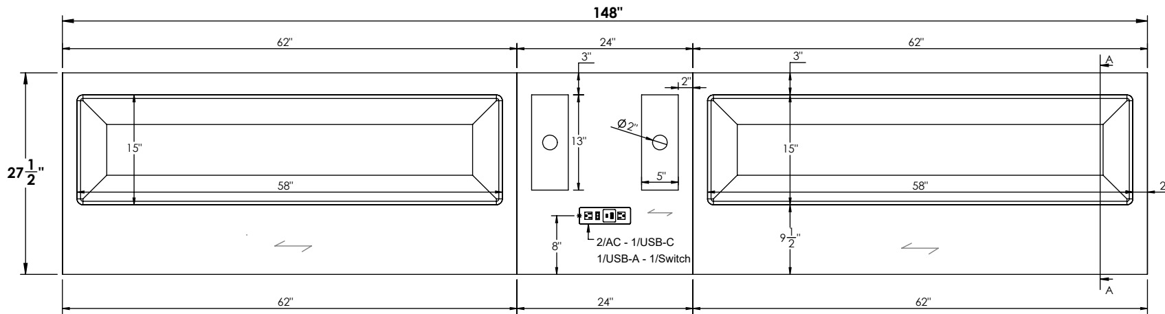
FRONT VIEW
